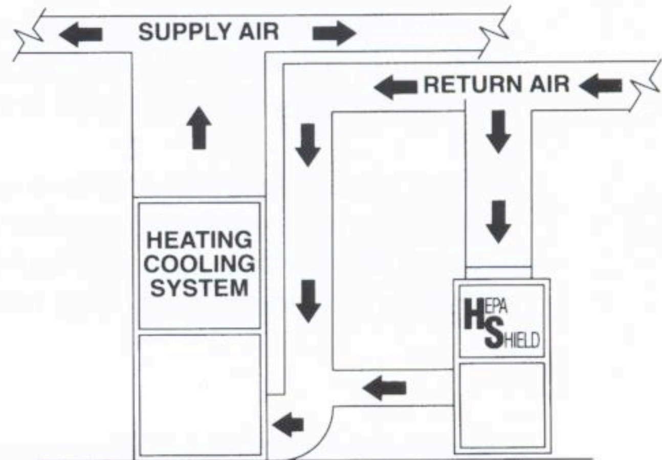
Typical Air Flow
